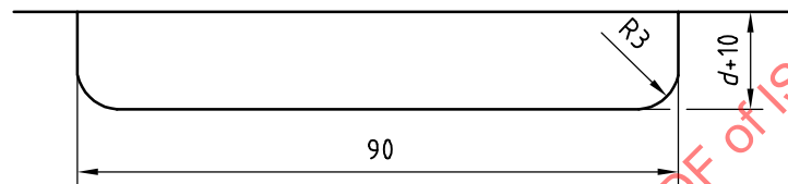
b) Dimensions of steel-bearing plate
