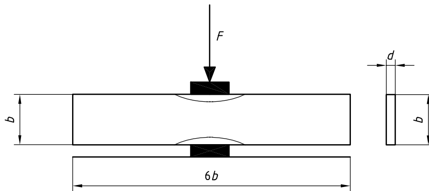
a) Loading configuration
