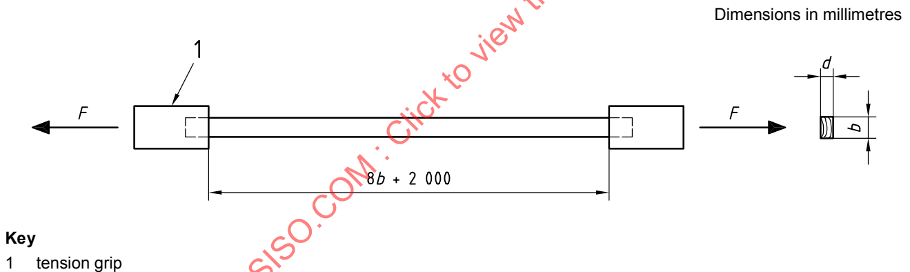
Figure 2 — Test set-up for measuring tension strength parallel to the grain
