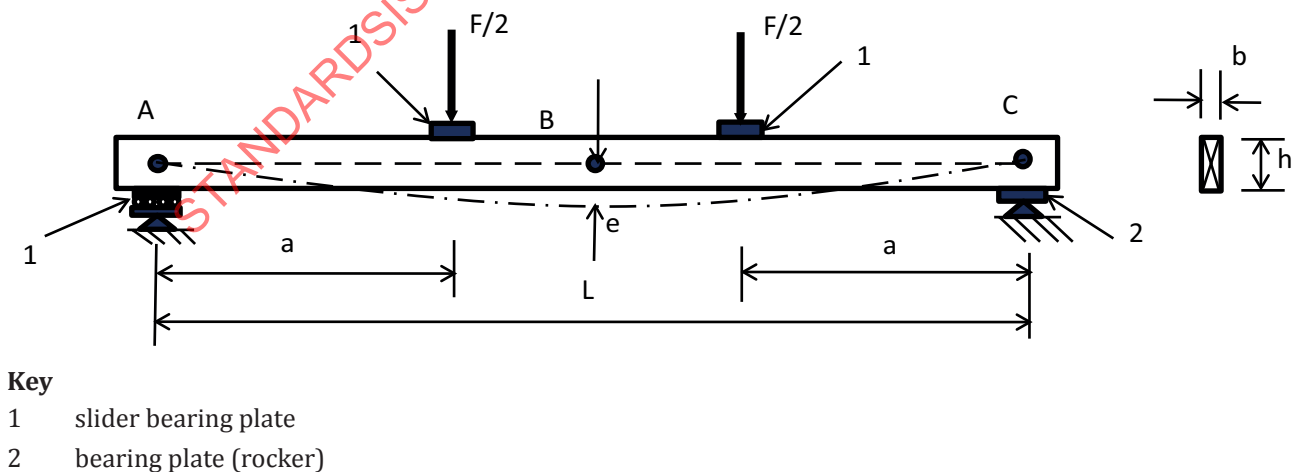
Figure 1 — Test set-up for measuring bending strength and stiffness
