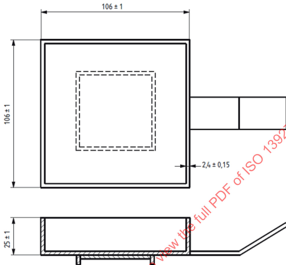
Figure 3 — Specimen holder
