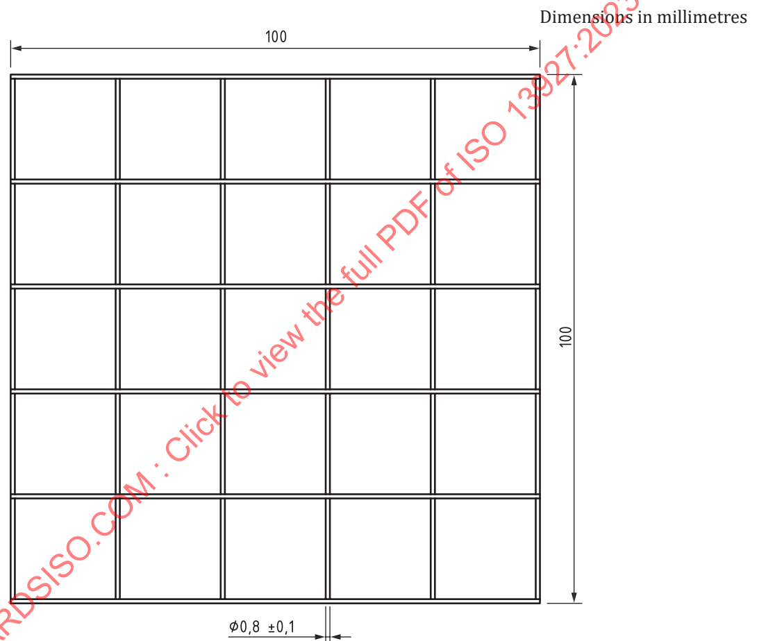
Figure 6 — Wire grid for use with dimensionally unstable materials
