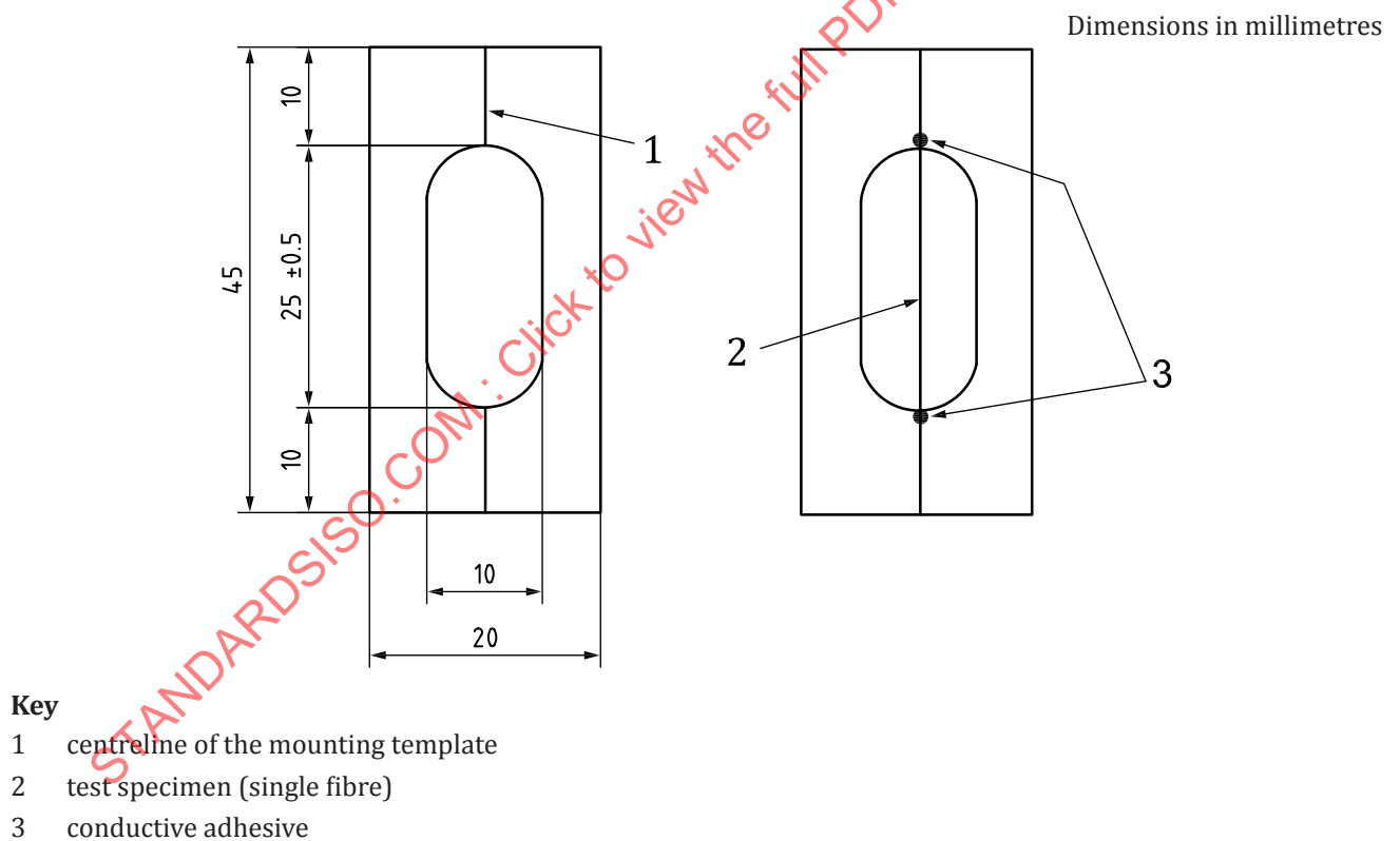
Figure 1 — Mounting tab for method A (for single filament)
