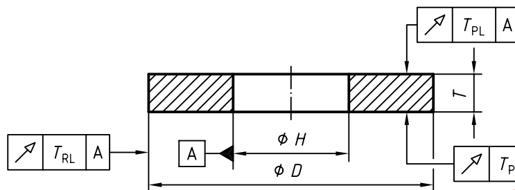
Figure 1 — Straight grinding wheel, e.g. as specified in ISO 603-1
