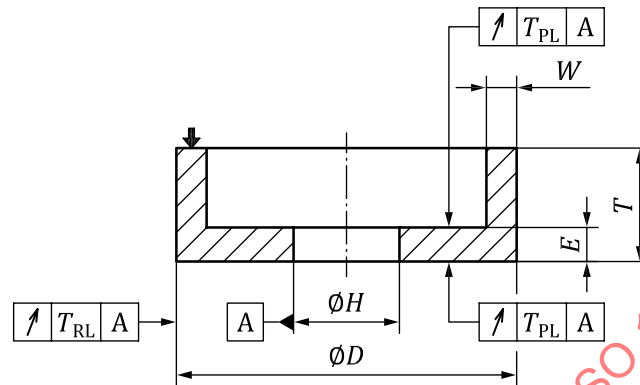
Figure 20 — Straight cup grinding wheel (Type 6)
