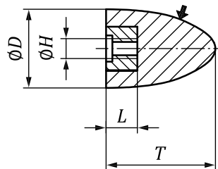
Figure 36 — Tapered grinding cone, curved, with threaded insert (Type 16)
