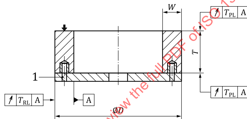
Figure 18 — Disc grinding wheel with threaded inserts, fixed to a back-plate (Type 36)
