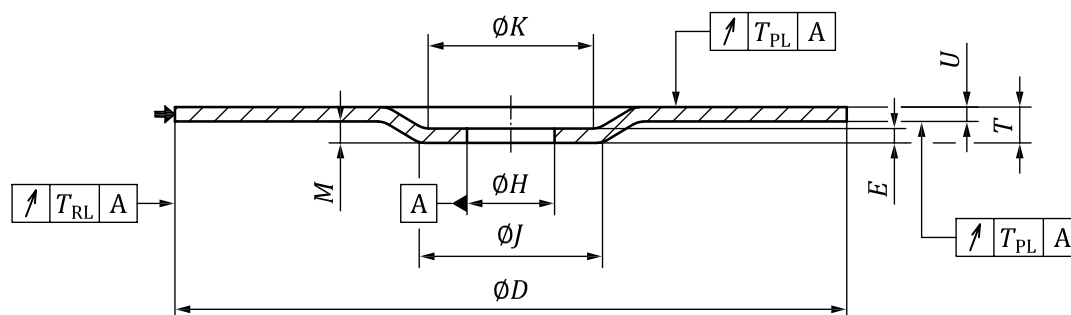
Figure 28 — Depressed centre cutting-off wheel (Type 42)
