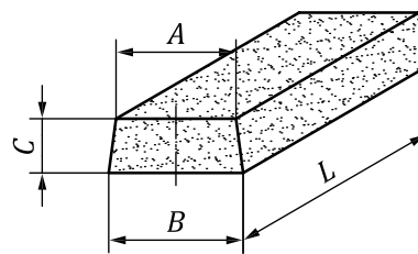
Figure 35 — Grinding segment, trapezoidal shape (Type 31G)
