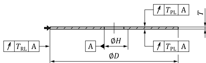
Figure 27 — Flat cutting-off wheel (Type 41)
