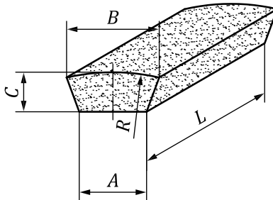
Figure 31 — Grinding segment, with outer radius (Type 31C)
