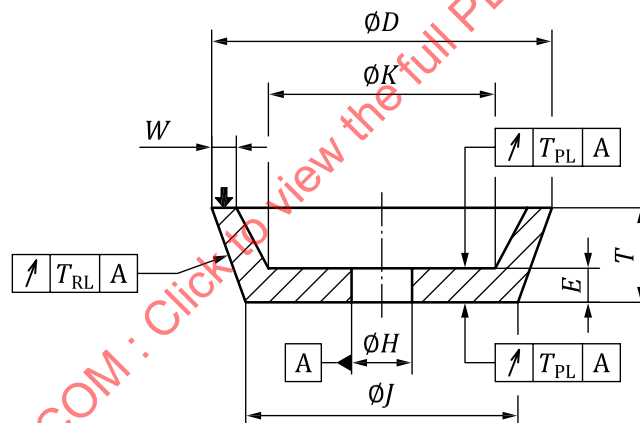
Figure 21 — Taper cup grinding wheel (Type 11)
