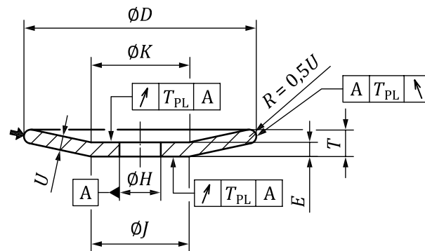
Figure 23 — Saucer grinding wheel (Type 13)
