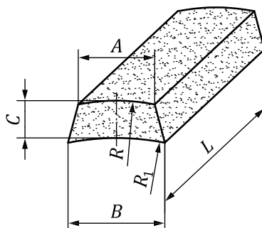
Figure 33 — Grinding segment, trapezoidal shape, with outer and inner radius (Type 31E)
