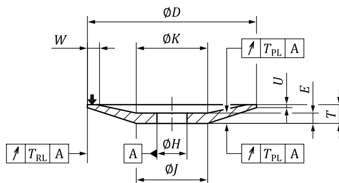
Figure 22 — Dish grinding wheel (Type 12)
