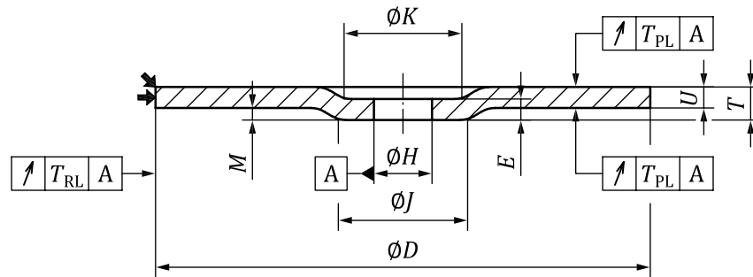
Figure 24 — Depressed centre grinding wheel for grinding or grinding/cutting-off (Type 27)
