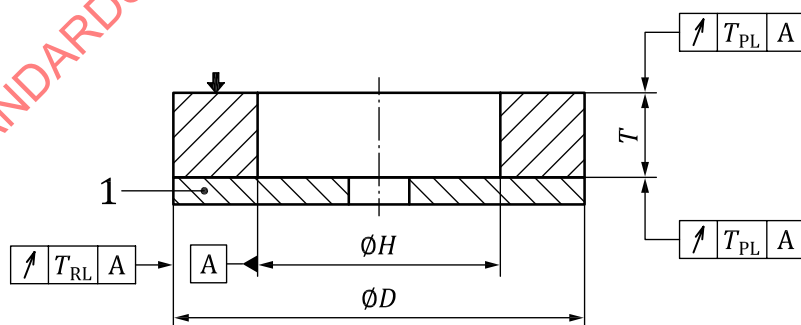
Figure 16 — Cylinder grinding wheel, cemented or clamped to a back-plate (Type 2)
