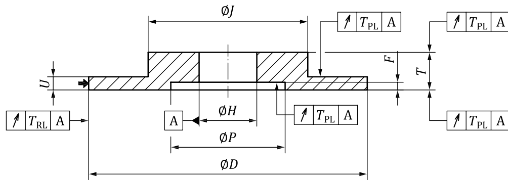
Figure 15 — Grinding wheel, hubbed on one side, recessed on the other side (Type 40)
