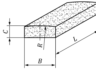
Figure 34 — Grinding segment, rectangular shape, with outer radius (Type 31F)
