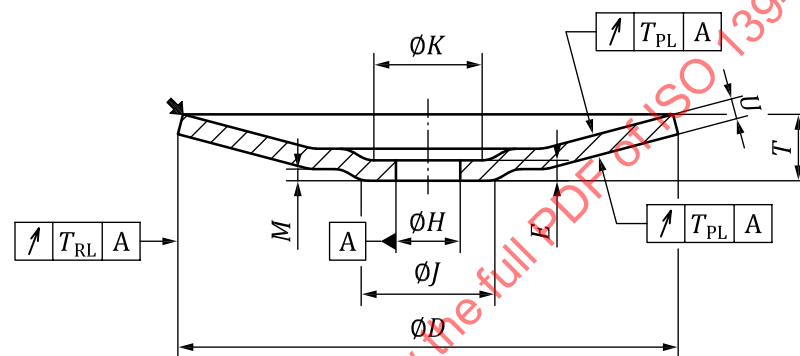
Figure 25 — Depressed centre grinding wheel, concave shaped (Type 28)
