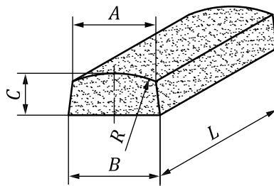
Figure 30 — Grinding segment, trapezoidal shape, with outer radius (Type 31B)
