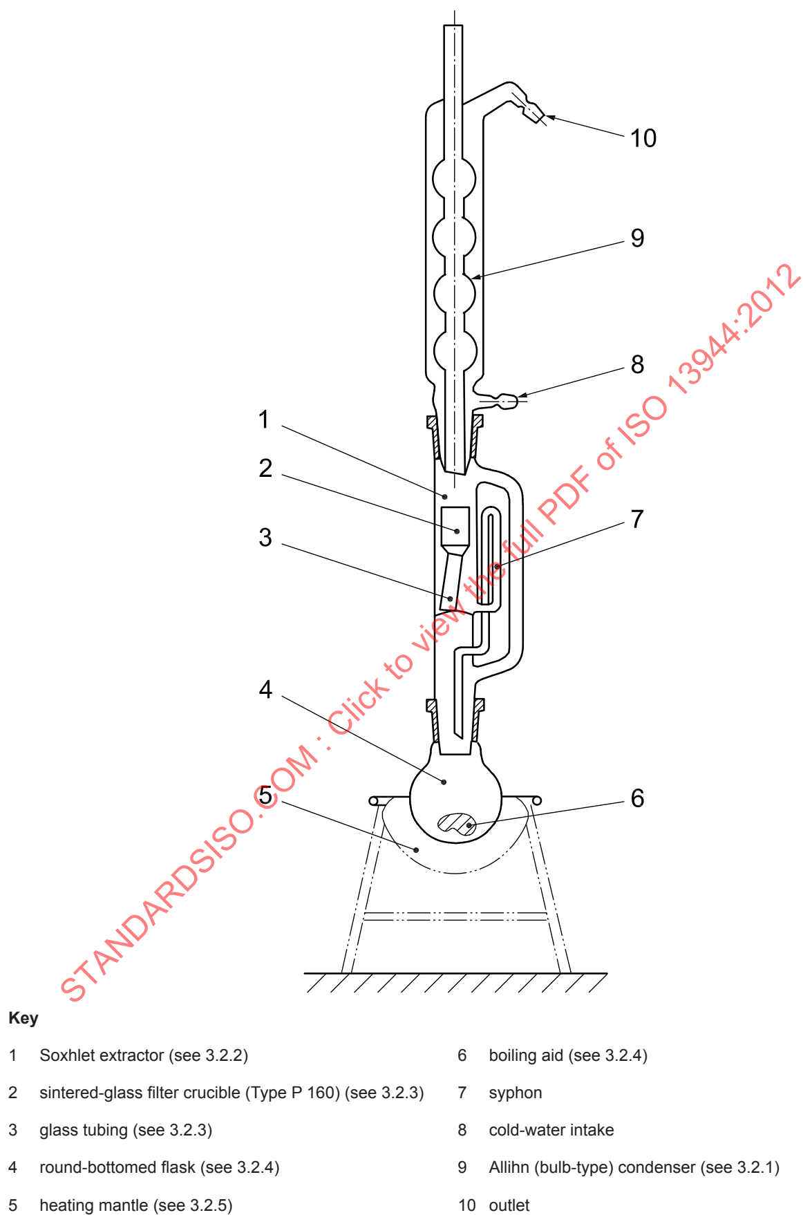
Figure 1 — Soxhlet apparatus (3.2)
