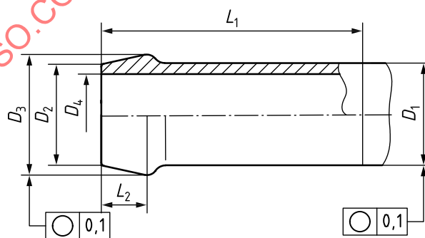
Figure 4 — Nipple, type A.1
