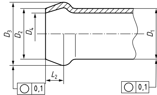
Figure 5 — Nipple, type A.2.1
