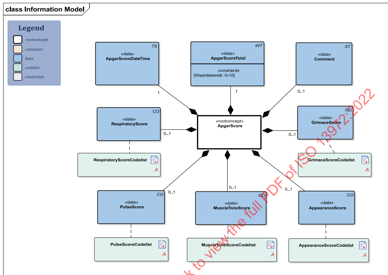
Figure 8 — Logical Model of the Apgar Score illustrating data elements as classes and references to value sets
