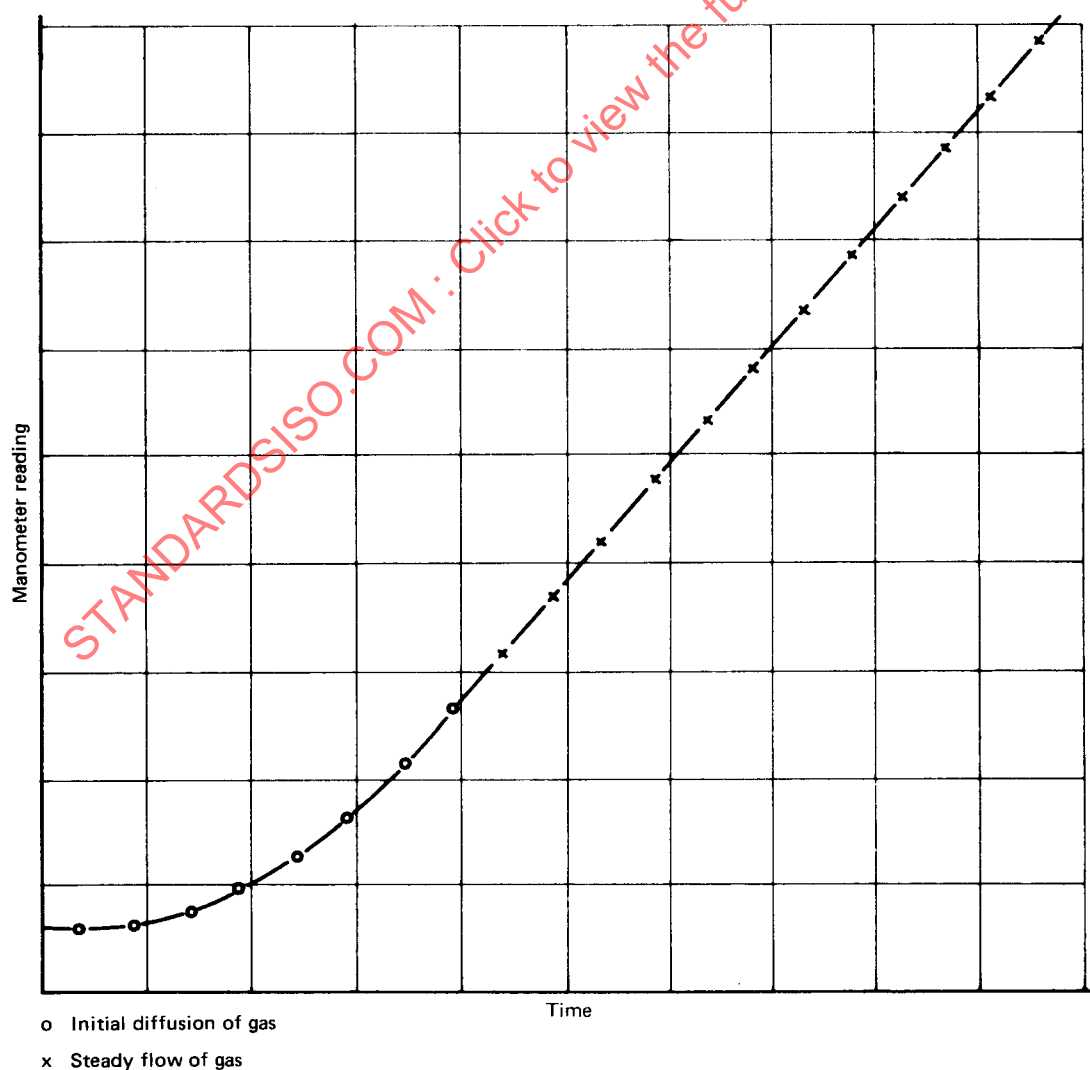
FIGURE 3 — Typical time/manometer reading curve
