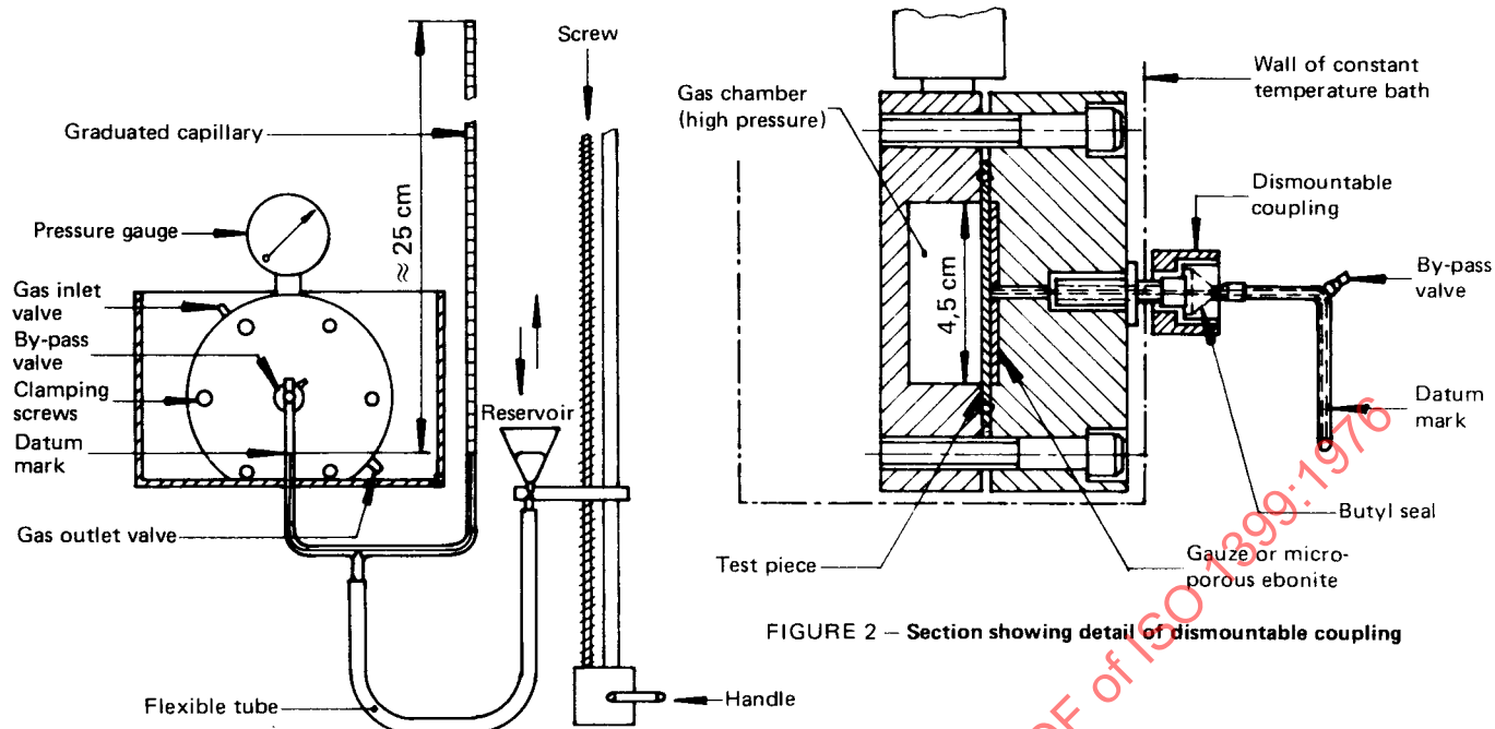
FIGURE 1 — Permeability apparatus
