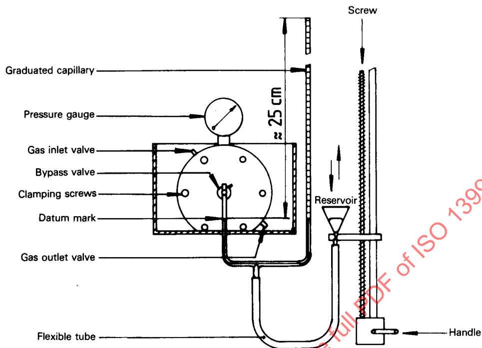
Figure 1 — Permeability apparatus
