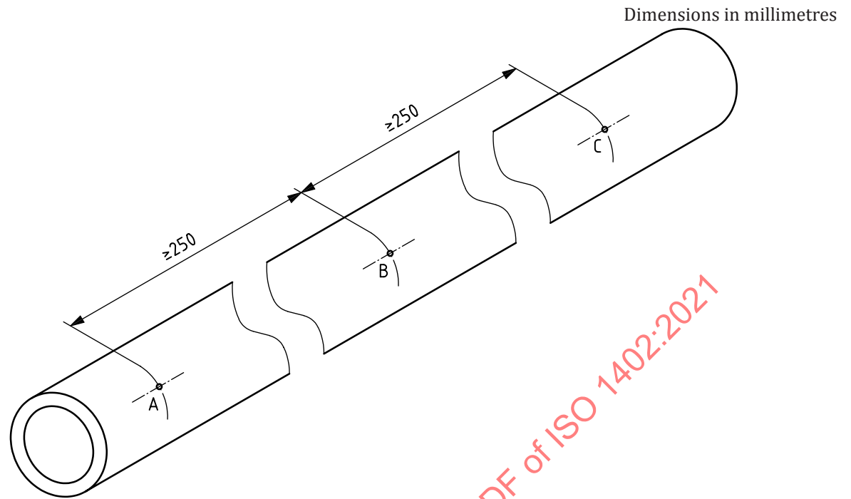
Figure 1 — Measurement of dimensional stability
