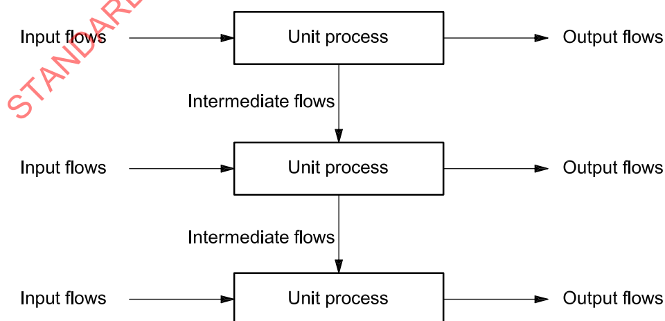
Figure 3 — Example of a set of unit processes within a product system
