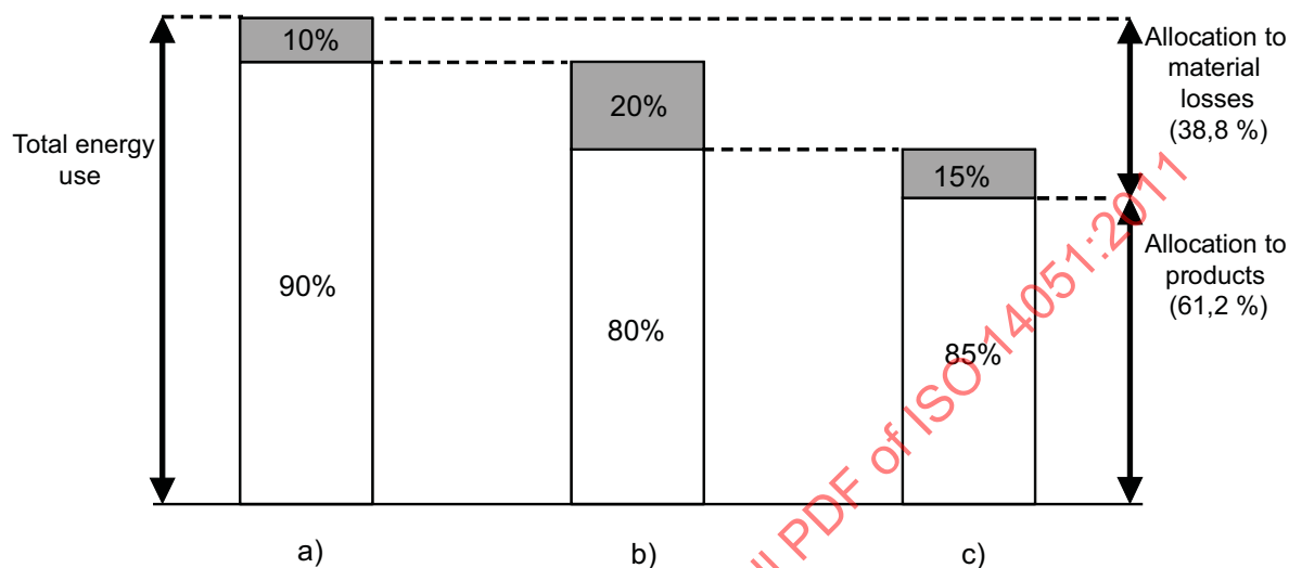
Figure B.3 — Quantification of energy loss
