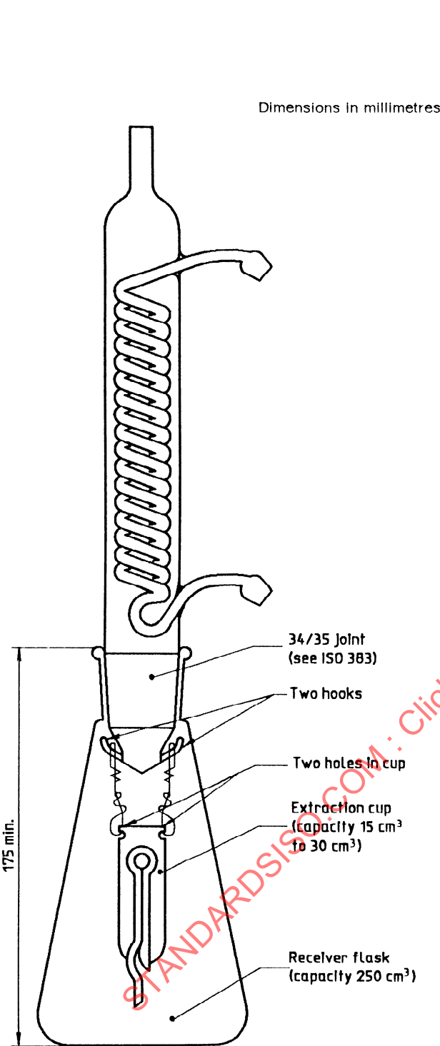
Figure 2 — Type 2 all-glass extraction apparatus
