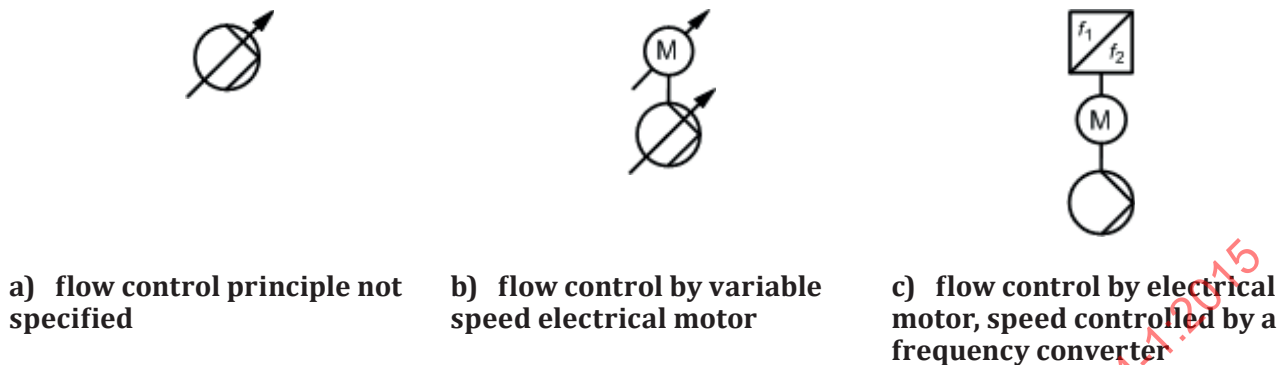
Figure 6 — Examples of different degrees of detailing of a variable flow pump
