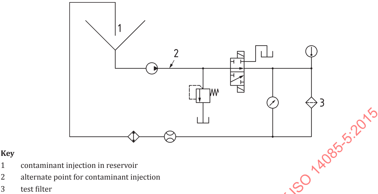
Figure 2 — Typical filter element flow fatigue cycle test stand circuit
