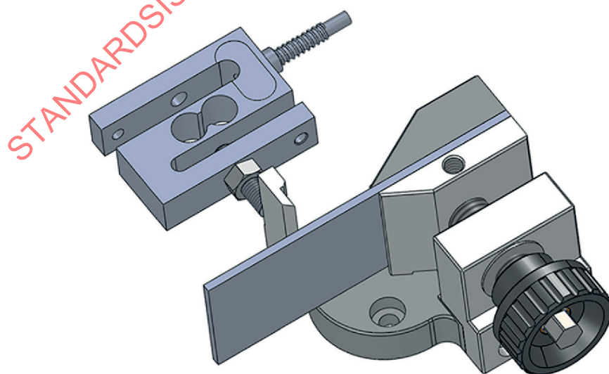
Figure 3 — 3D drawing of clamping jaws with specimen, load cell and bar
