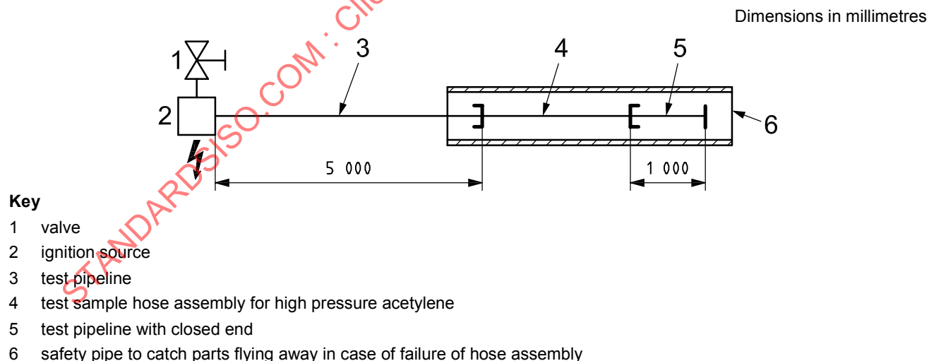
Figure A.1 — Test assembly for acetylene decomposition test with hose assembly for high pressure acetylene
