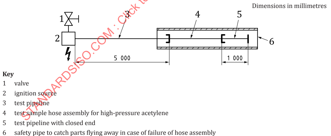
Figure A.1 — Test assembly for acetylene decomposition test with hose assembly for high-pressure acetylene
