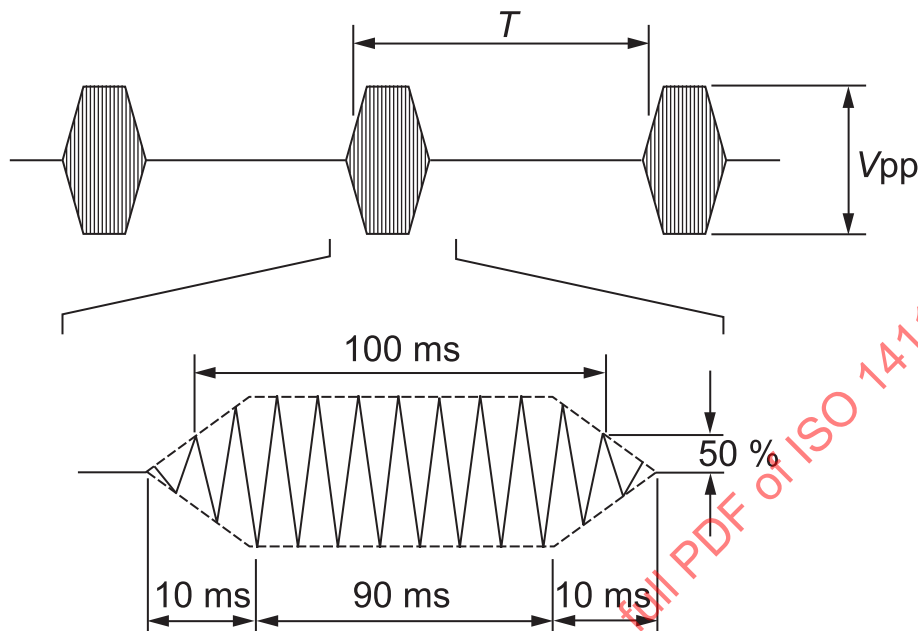
Figure 34 — Test signal 2 : Modulation 2 (preferred) in the range of 1 kHz to 150 kHz
