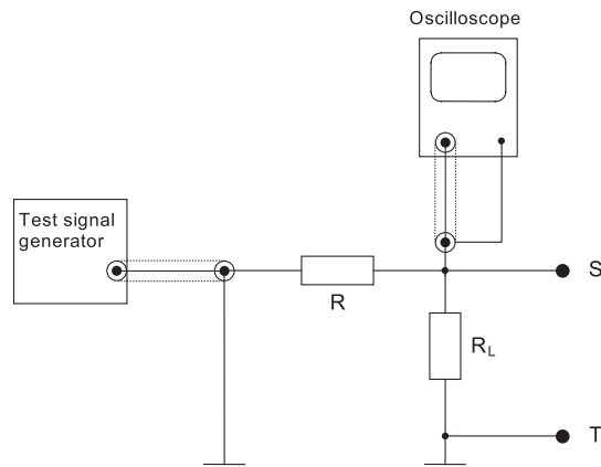
Figure 42 — Test setup for magnetostatic measurements
