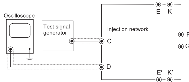
Figure 21 — Test setup to check for malfunction at high frequency
