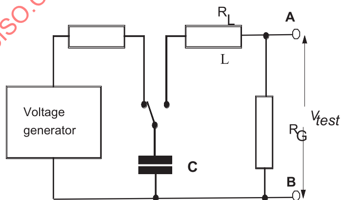
Figure 46 — Circuit for generating a damped sinus defibrillation waveform for Test 1
