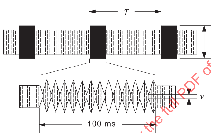
Figure 20 — Test signal for frequencies between 10 MHz and 450 MHz
