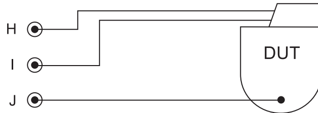
Figure 16 — Common mode connection to a single-channel bipolar device
