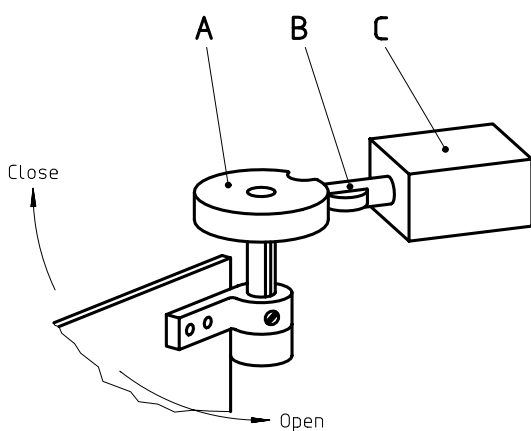
Figure A.1 — With a rotating guard
