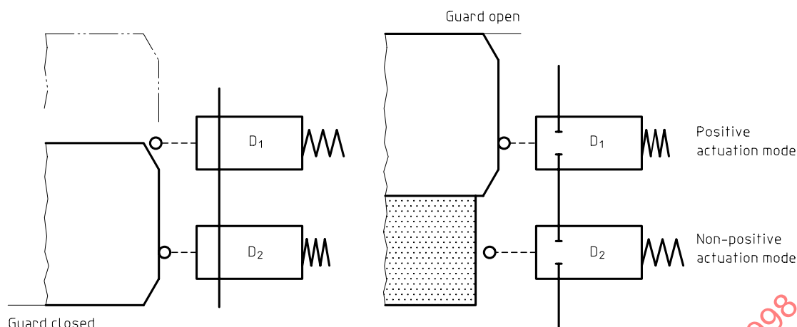
Figure 4 — Avoiding common-cause failure of two mechanically actuated position detectors by using associated positive and non-positive mode actuation
