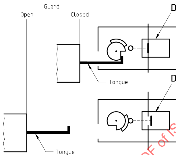
Figure B.1 — Device with tongue-operated switch
