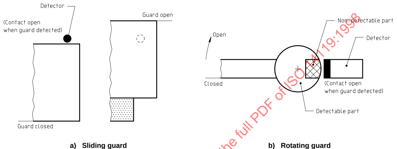
Figure 6 — Examples of protection against defeat of a proximity switch or magnetic switch
