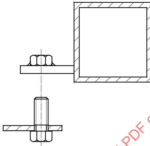
Figure 11 — Example of a retained fastening
