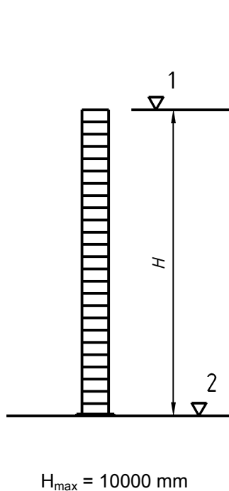
Figure 1.a : Ladder without rest platform (single flight)
