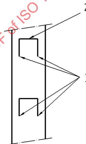
Figure 6.b — Design of polygonal rungs — Recommended mounting
