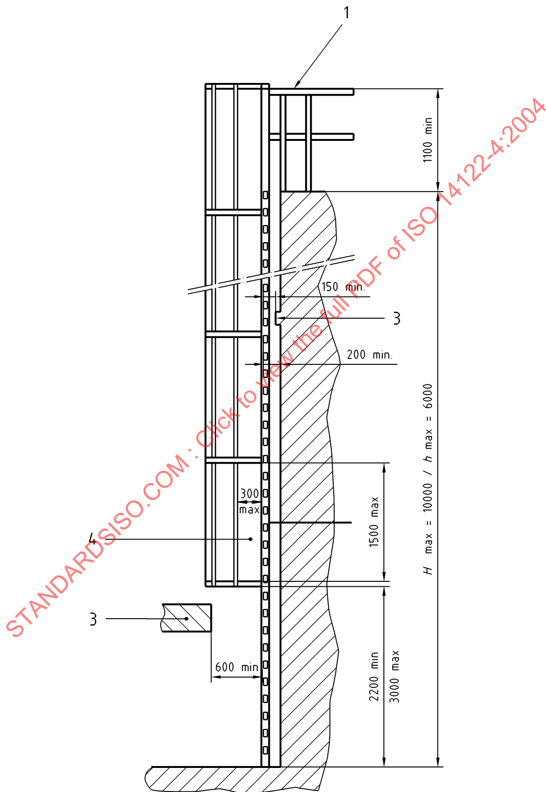
Figure 4a — Side elevation on ladder with a safety cage
