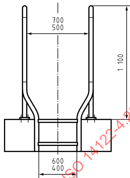
b) Example for cranked stiles
