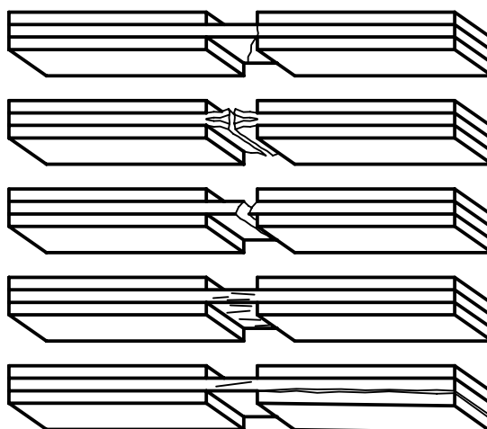
Figure 6 — Acceptable modes of failure
