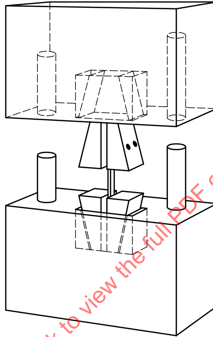
Figure C.1 — ASTM D 3410/B [2]
