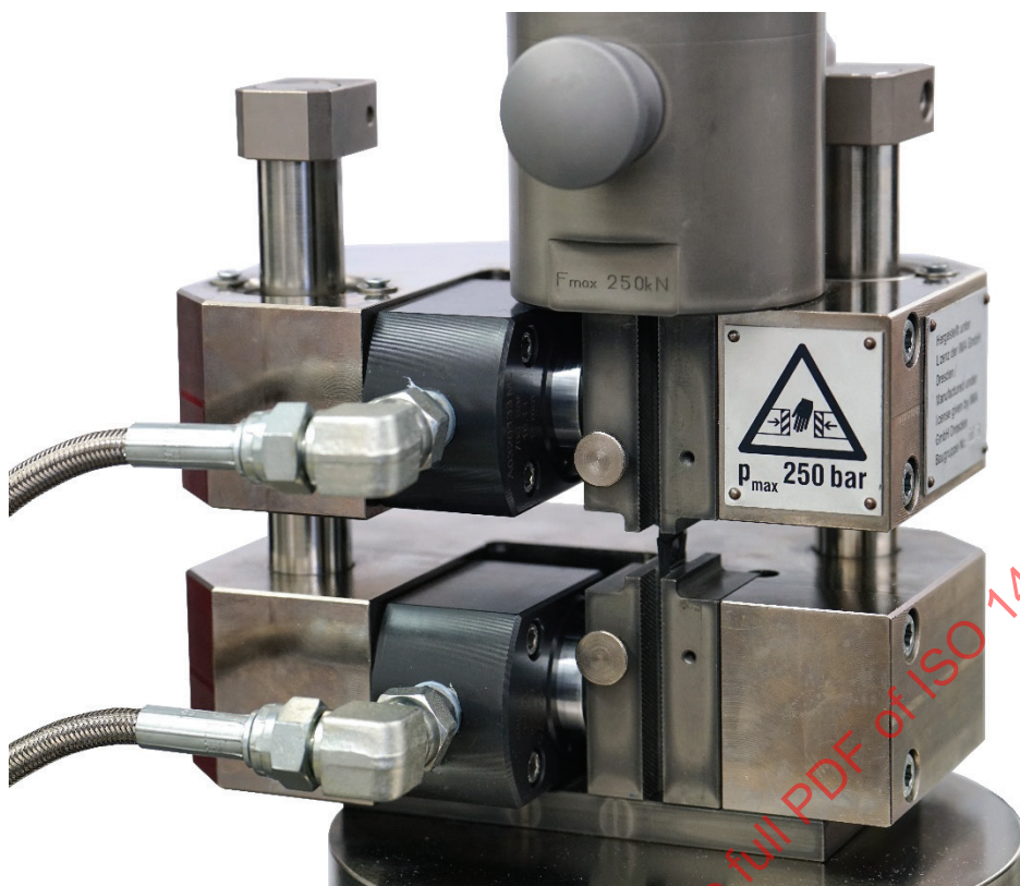
Figure D.6 — Hydraulic composites compression fixture (HCCF)
