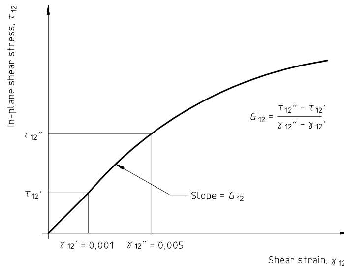
Figure 3 — Shear stress/shear strain diagram
