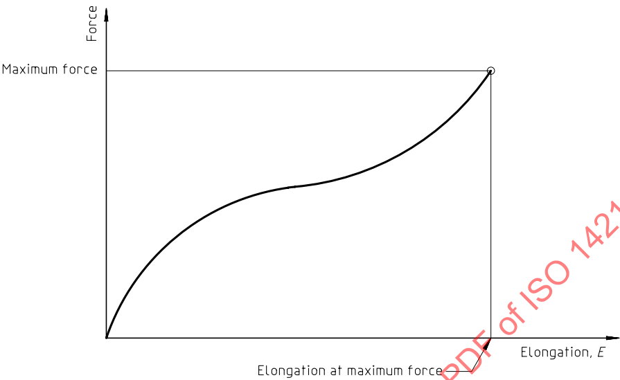
Figure 1 — Maximum force at break
