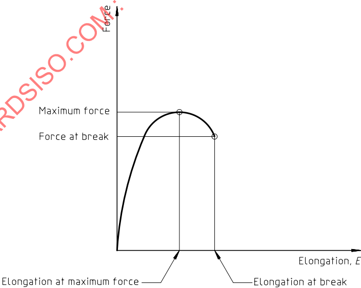
Figure 2 — Tensile force at break
