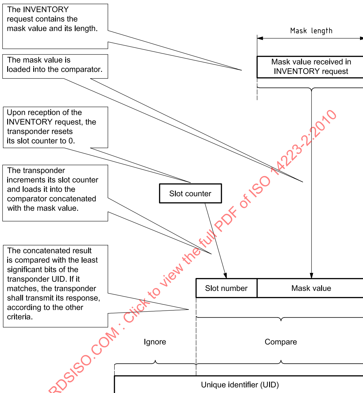
Figure 2 — Principle of comparison between mask value, slot number and UID
