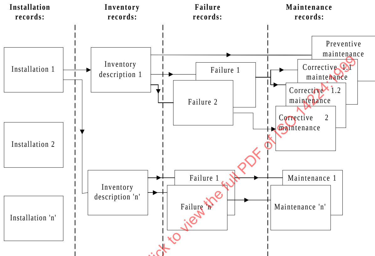
Figure 3 — Database structure
