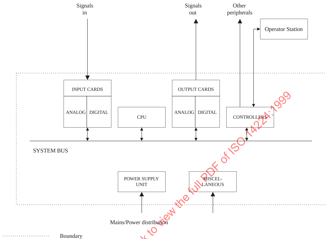
Figure A.3 — Equipment boundary — Control logic units
