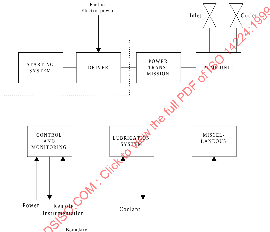
Figure 1 — Example of boundary diagram (pumps)
