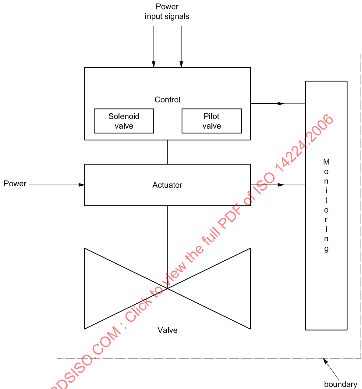
Figure A.22 — Boundary definition — Valves
