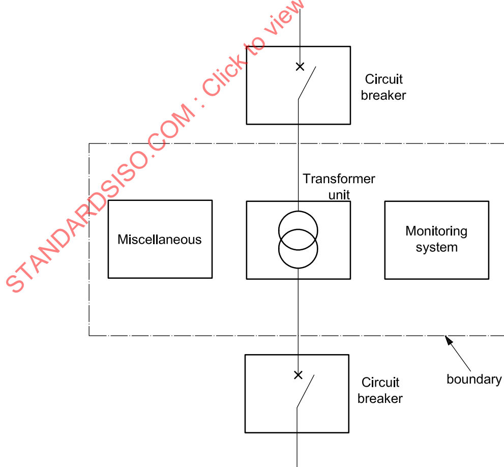
Figure A.18 — Boundary definition (typical) — Power transformer
