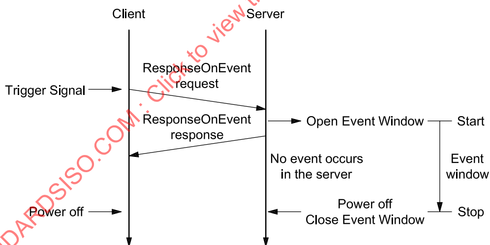
Figure 15 — Infinite event window — No event during active event window
