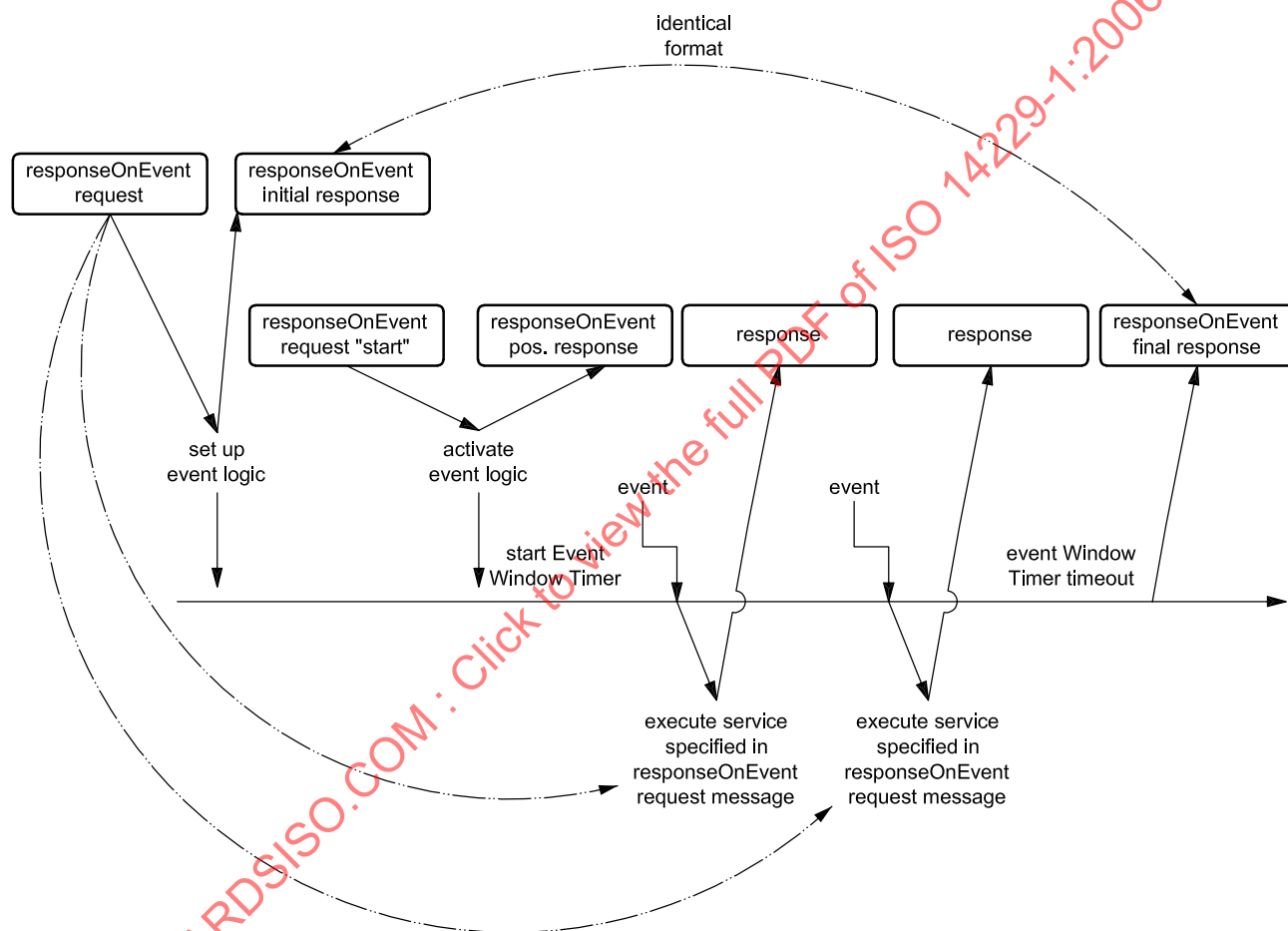
Figure 12 — ResponseOnEvent service — Client and server behaviour
