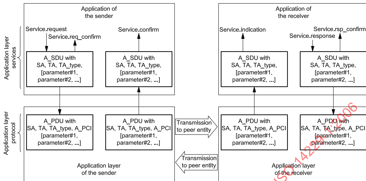
Figure 3 — The services and the protocol
