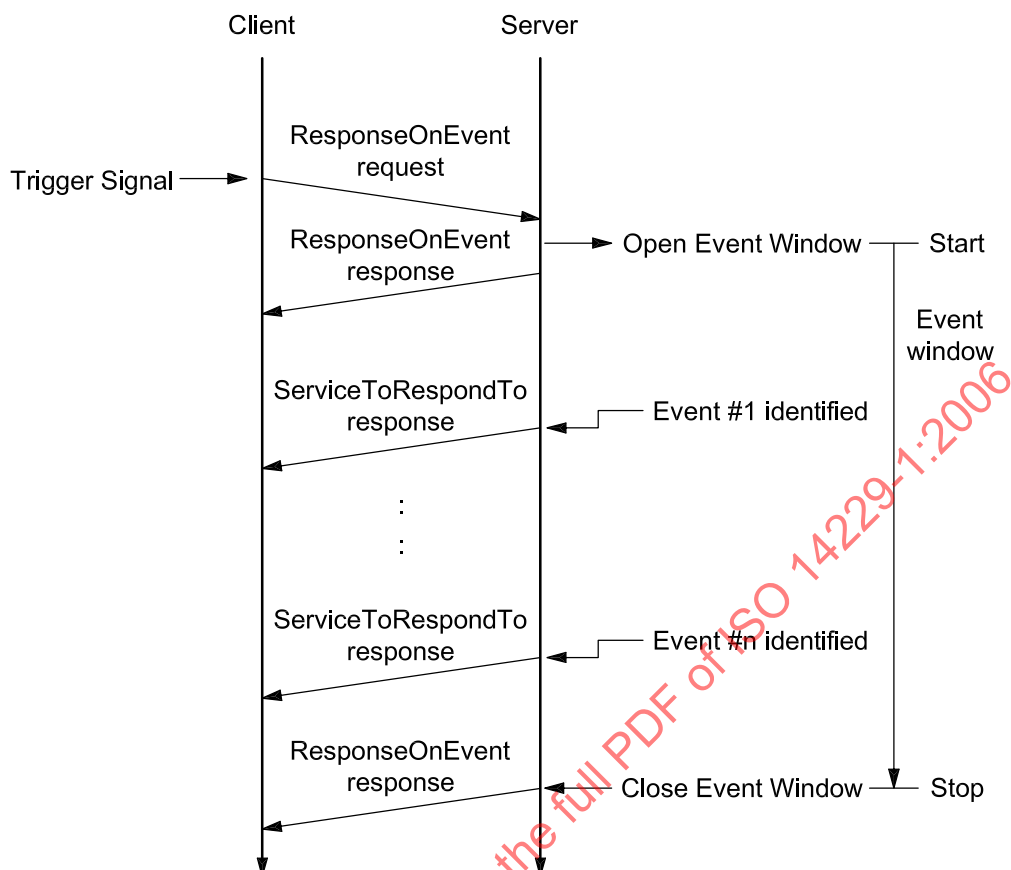
Figure 14 — Finite event window — Multiple events during active event window
