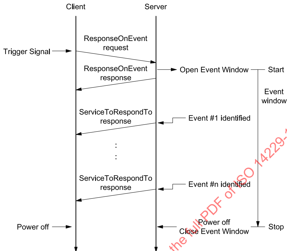
Figure 16 — Infinite event window — Multiple events during active event window
