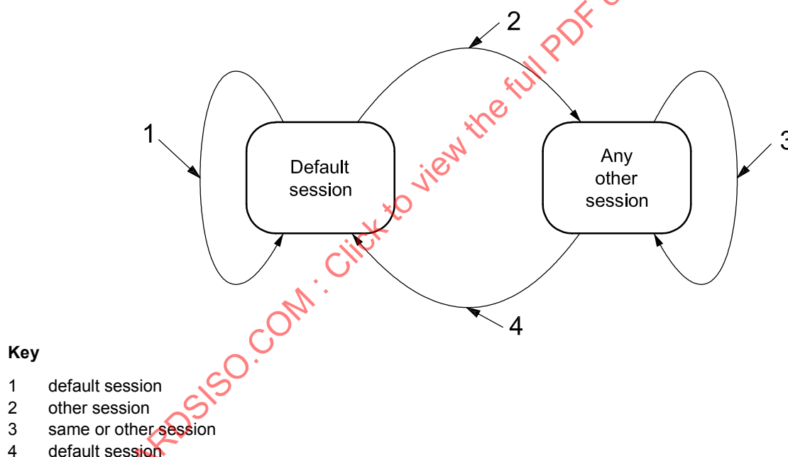
Figure 9 — Server diagnostic session state diagram
