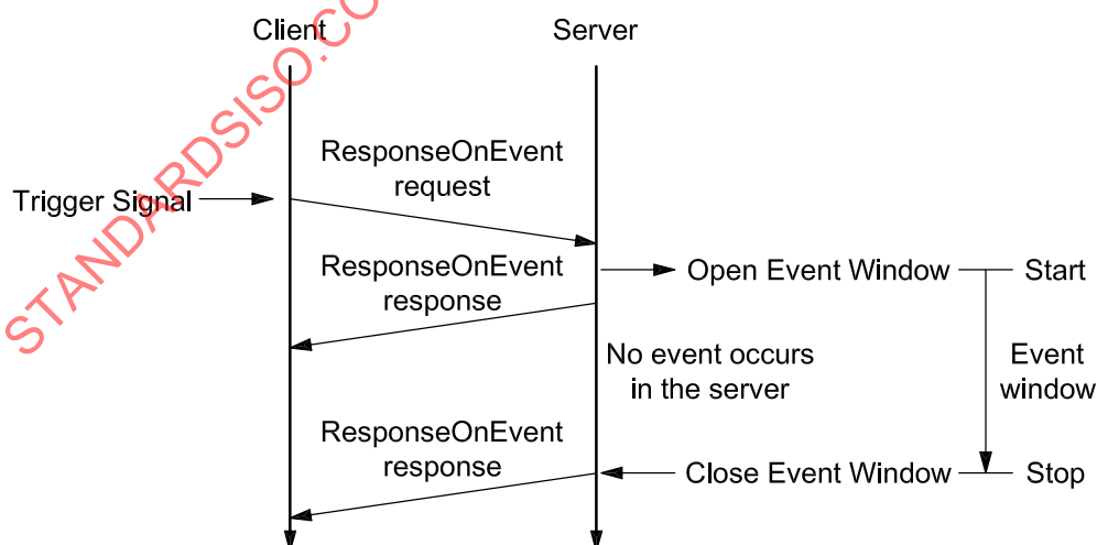
Figure 13 — Finite event window — No event during active event window
