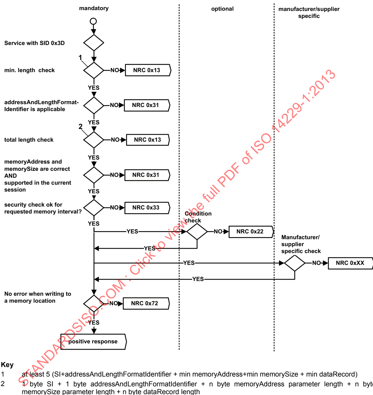
Figure 22 — NRC handling for WriteMemoryByAddress service
