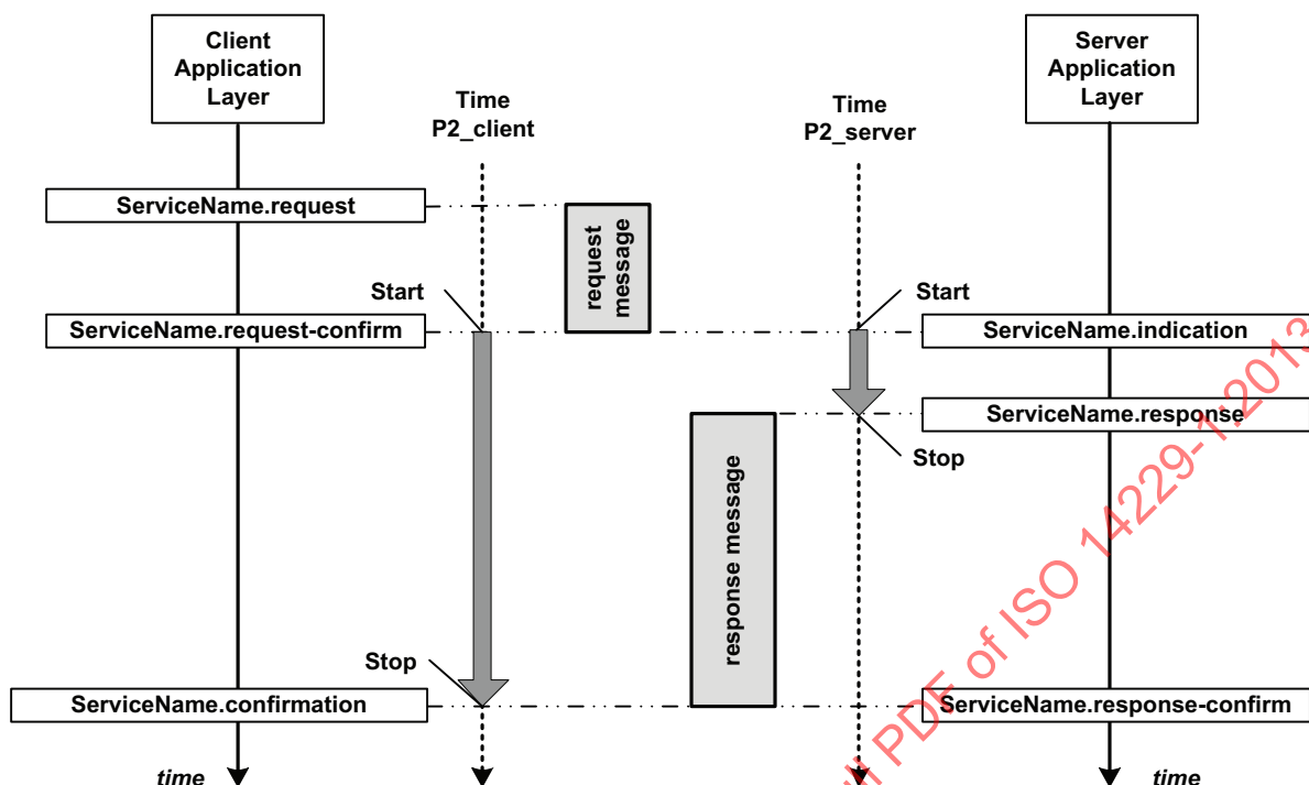
Figure 3 — Application layer service primitives - confirmed service
