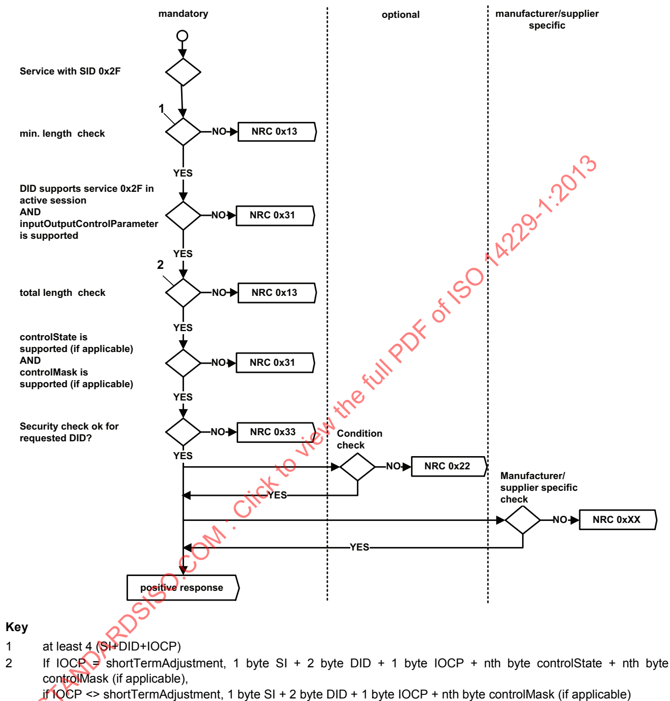
Figure 24 — NRC handling for InputOutputControlByIdentifier service
