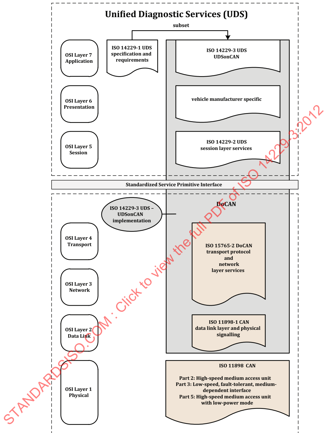
Figure 1 — UDSONCAN document reference according to OSI model
