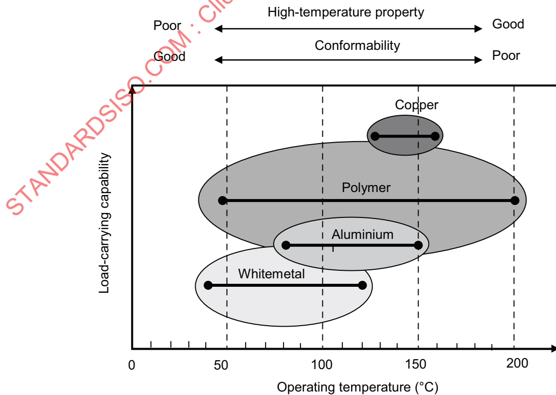
Figure A.2 — General chart concerning the operation range for metallic materials and polymer materials
