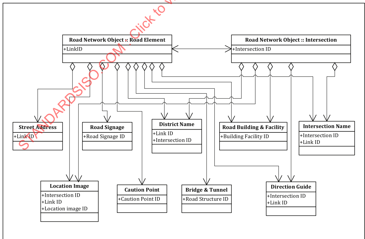
Figure 12 — Intersection and road element guidance package
