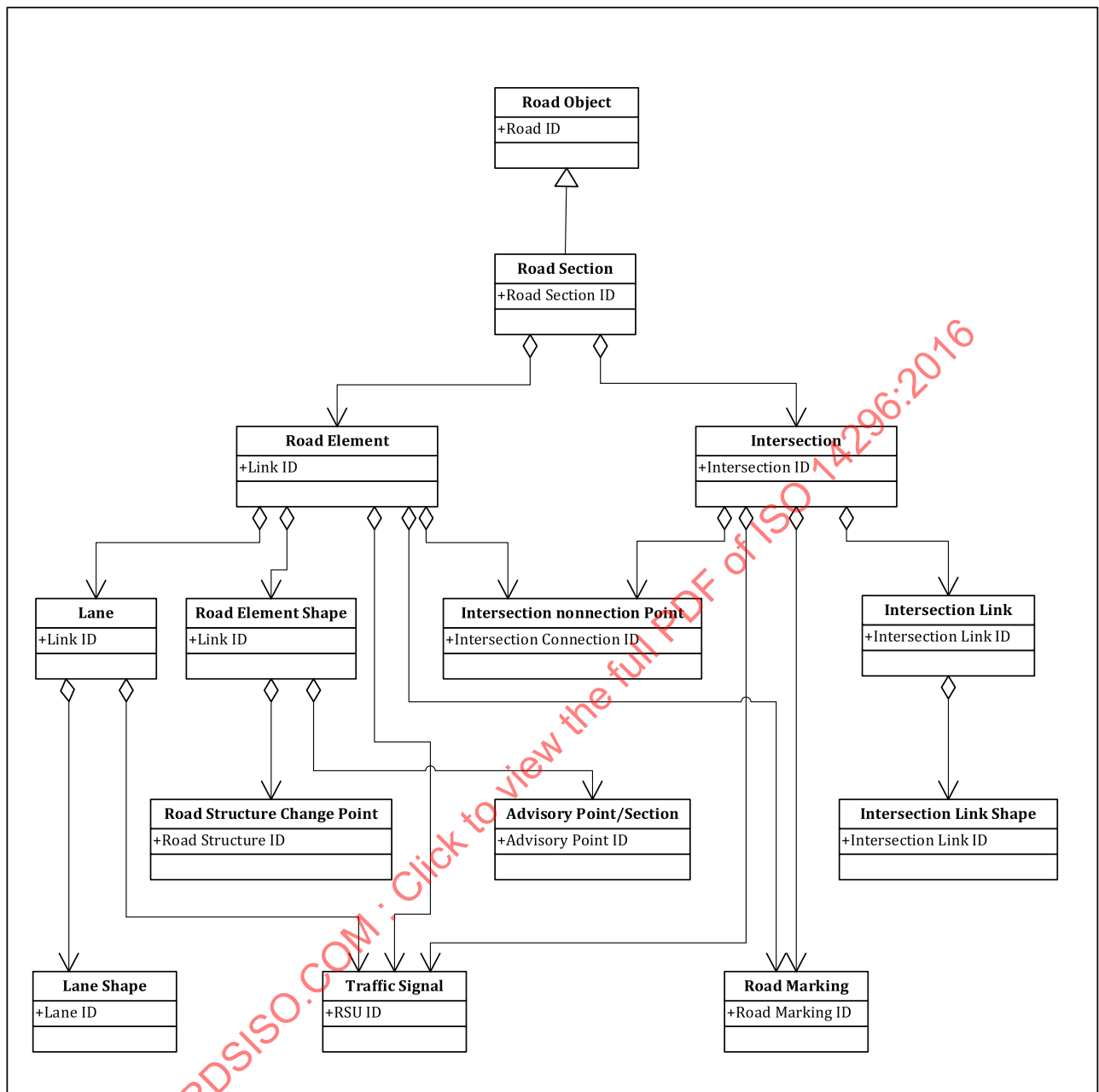
Figure 4 — Road network object package
