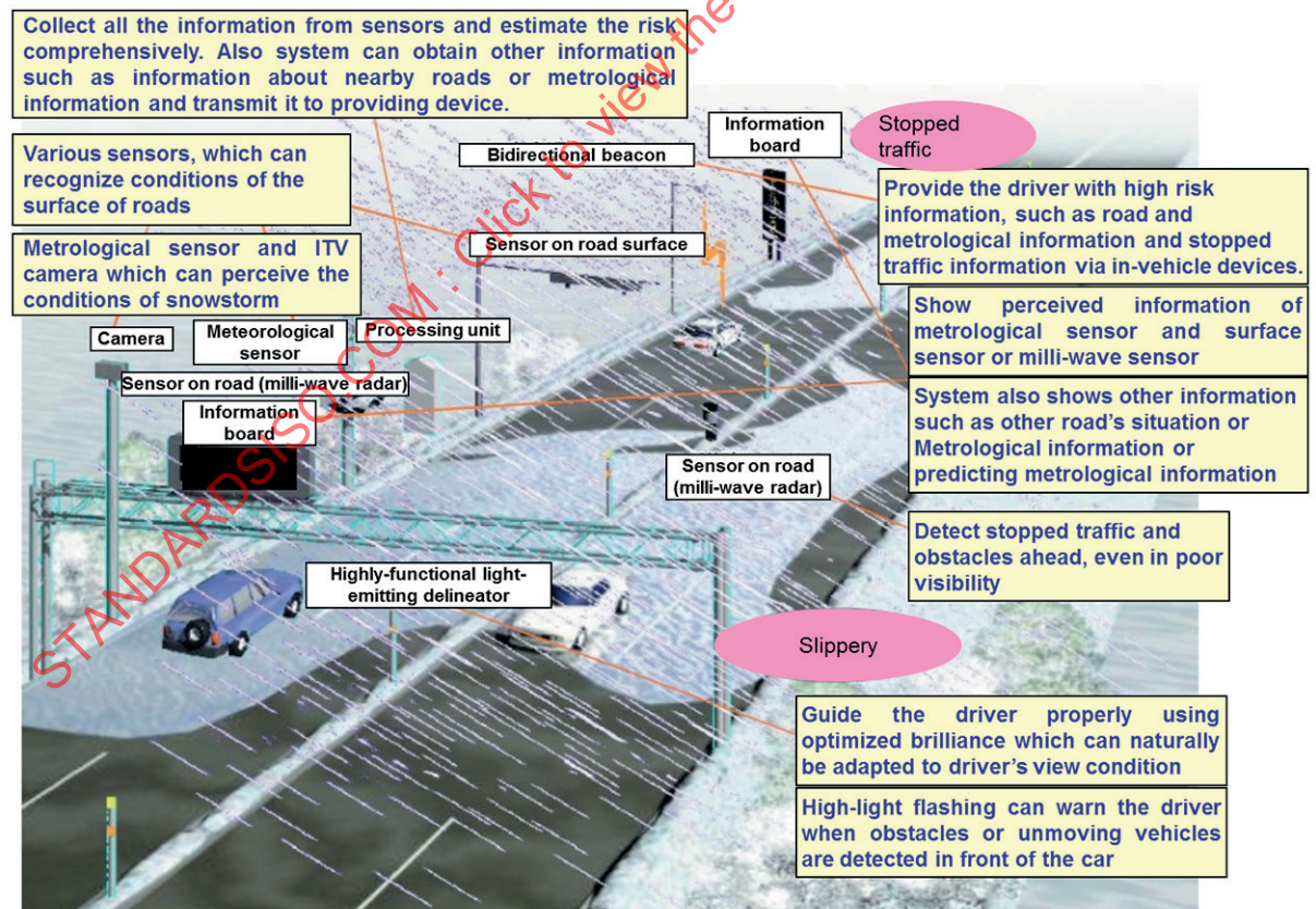
Figure D.9 — Road surface condition warning
