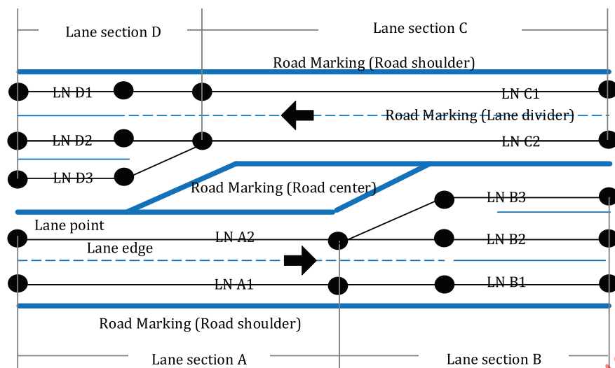
Figure 9 — Lane structure
