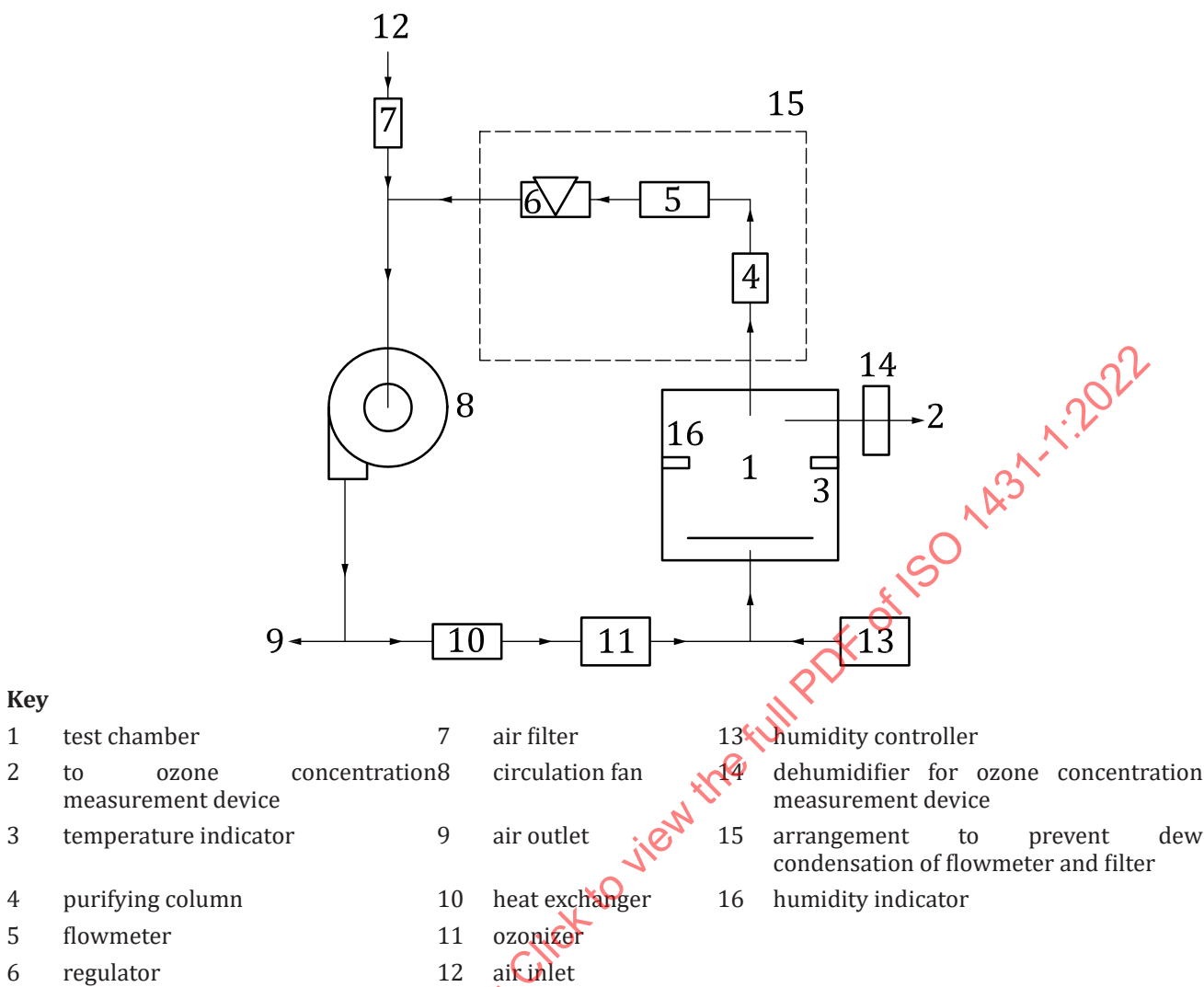
Figure 2 — Example of a test apparatus with humidity control
