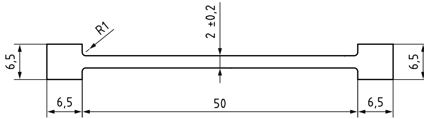
Figure 4 — Narrow strip test piece
