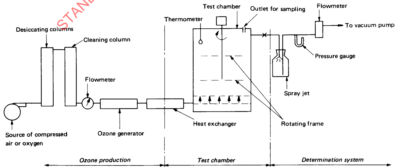
FIGURE 1 — Schematic diagram of apparatus for ozone cracking resistance test
