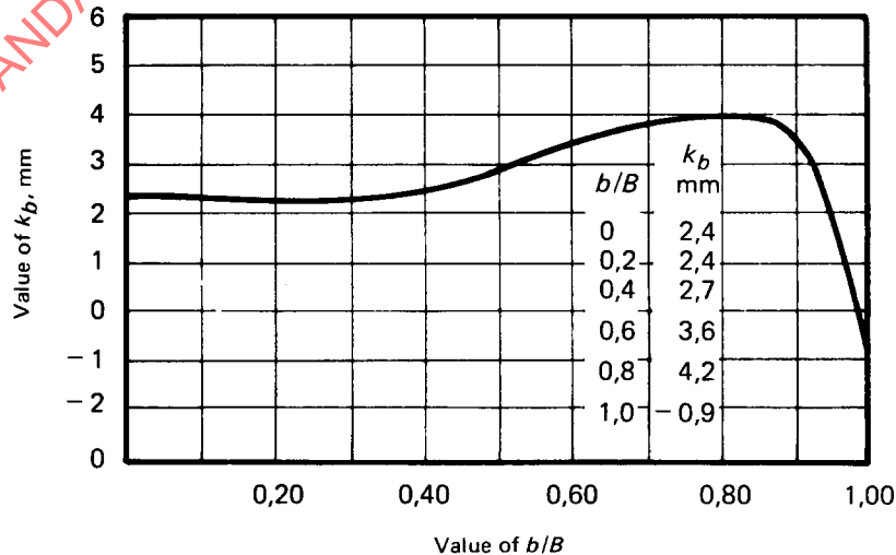
FIGURE 8 – Value of k_b related to b/B
