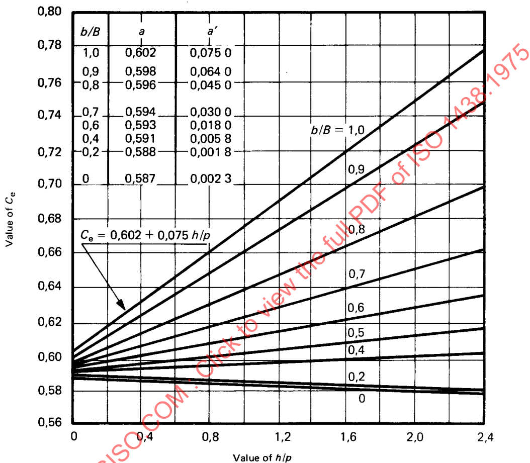
FIGURE 7 – Coefficient of discharge C_e
