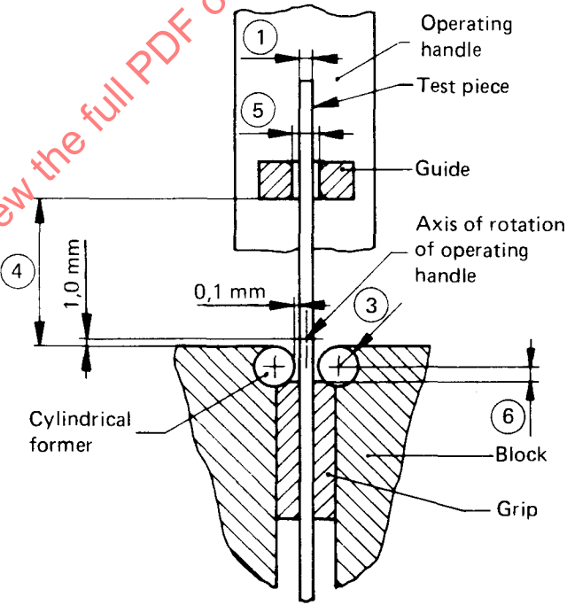
FIGURE 1 — Essential elements of bend testing machine for wire
