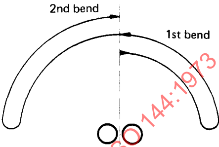
FIGURE 2 – Method of counting bends
