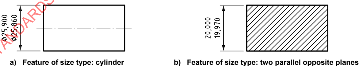
Figure 11 — Example: ISO basic GPS specification of size — Values of upper and lower limits of size (ULS and LLS)
