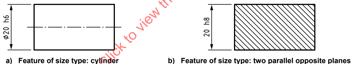
Figure 10 — Example: ISO basic GPS specification of size — Nominal size followed by ISO tolerance code — ISO 286-1
