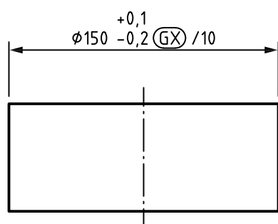
a) By using the / length symbol
