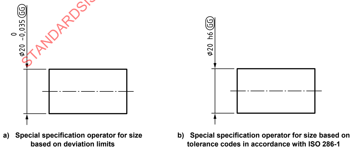
Figure 15 — Example: Indication of a special specification operator for size
