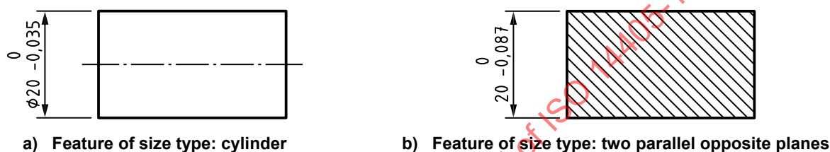
Figure 9 — Example: ISO basic GPS specification of size — Nominal size \pm deviation limits
