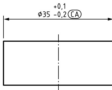
Figure 16 — Example: Same specification operator for upper limit of size and lower limit of size
