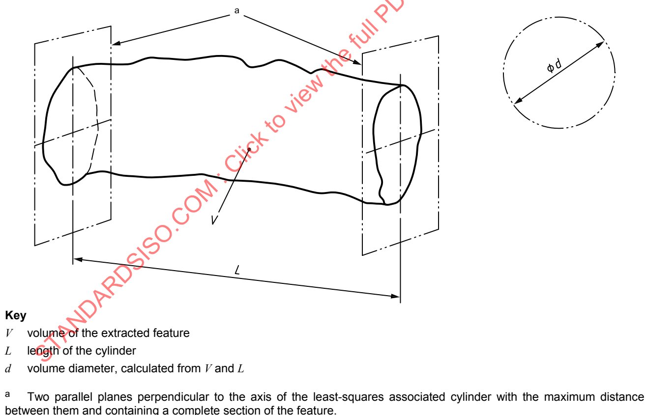
Figure 7 — Example of volume diameter
