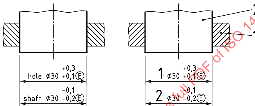
Figure 14 — Examples of assembly drawing with plus and minus tolerancing of two features in a fit
