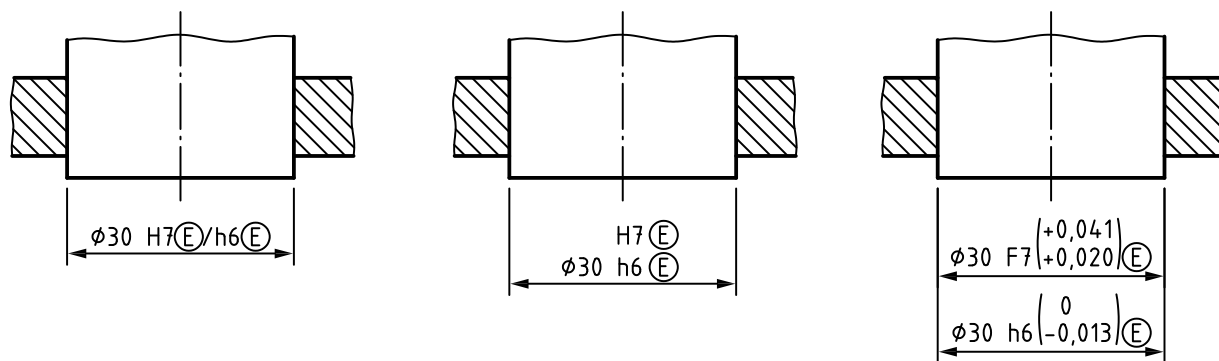
Figure 13 — Examples of assembly drawing with ISO code system tolerancing of two features in a fit
