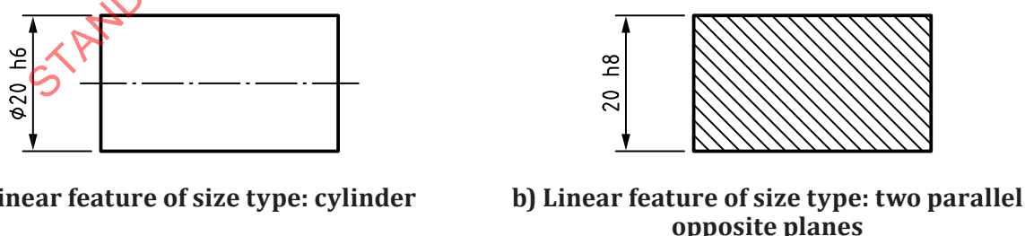
Figure 12 — Example of ISO basic GPS specification of size — Nominal size followed by ISO tolerance code — ISO 286-1
