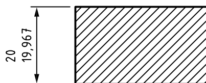
b) Linear feature of size type: two parallel opposite planes
