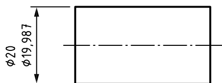
a) Linear feature of size type: cylinder
