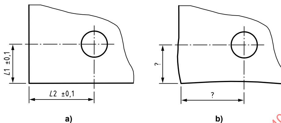
Figure A.8 — Example of linear distance in two directions
