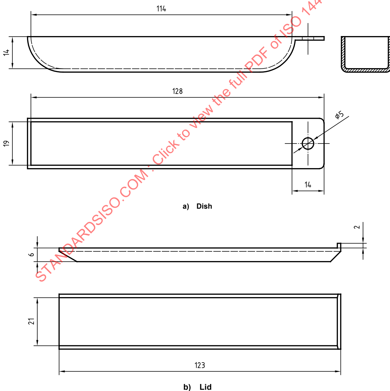
Figure A.1 — Diagram of suitable metal dish and lid (for guidance only)
