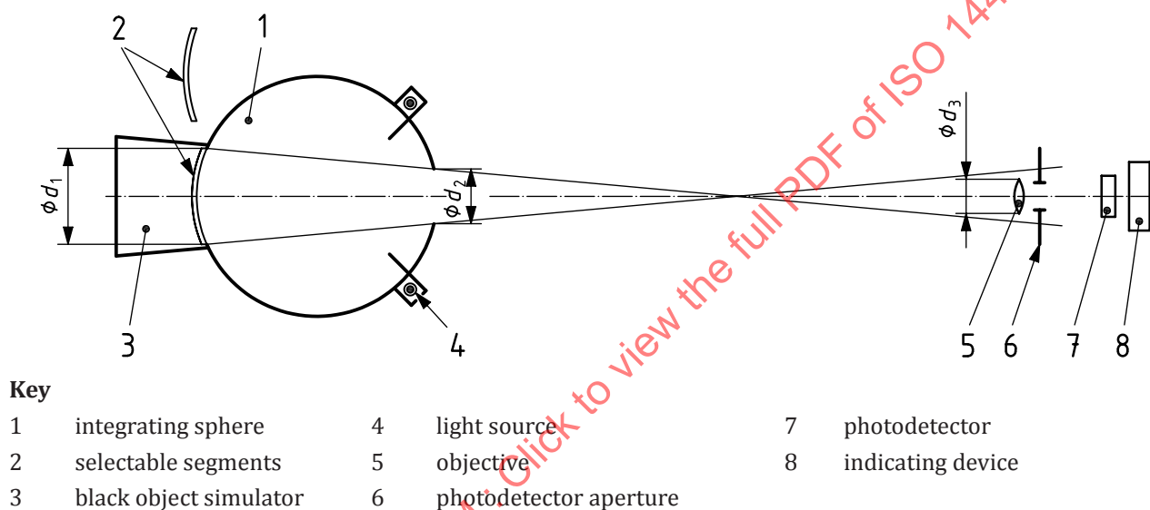
Figure A.1 — Arrangement for determination of the luminance ratio (schematic)
