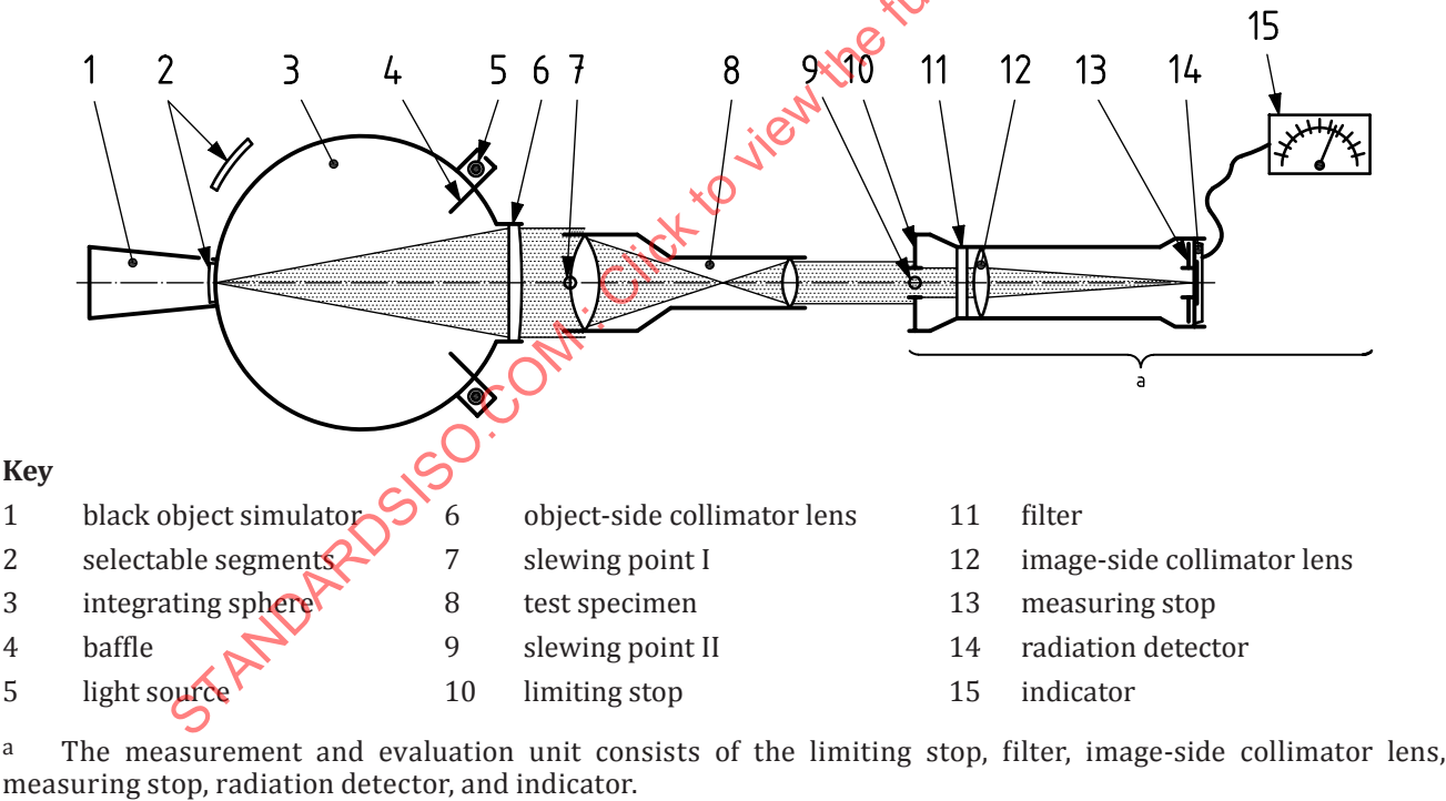
Figure 1 — Test arrangement for on-axis measurement (schematic)
