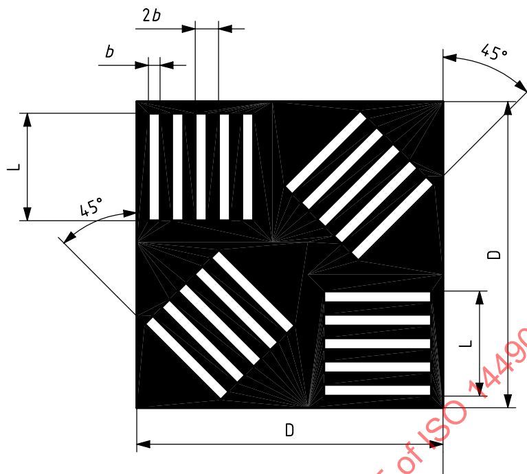
Figure A.2 — A group of the resolution test target
