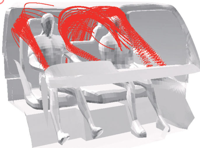
Figure B.3 — Stream line of air conditioning flow in the cabin
