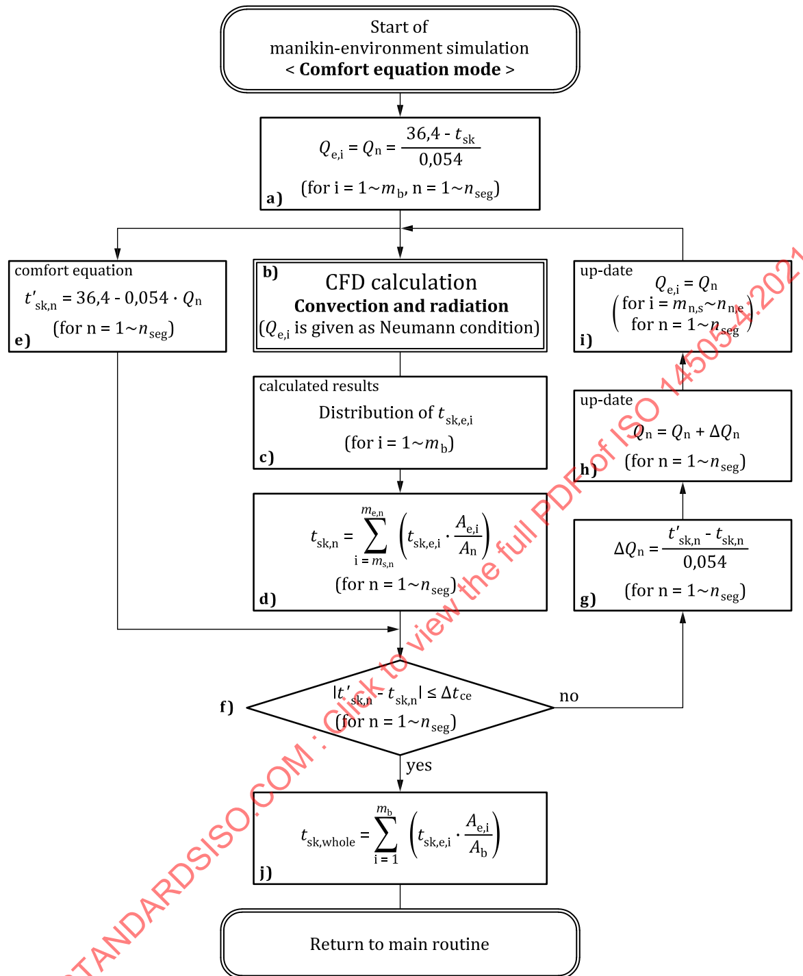
Figure E.4 — Algorithm for the comfort equation mode
