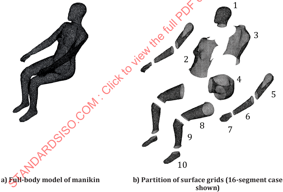
Figure 4 — Theoretical structure of numerical manikin
