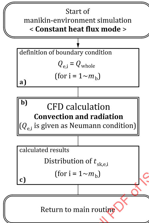
Figure E.3 — Algorithm for the constant heat flux mode
