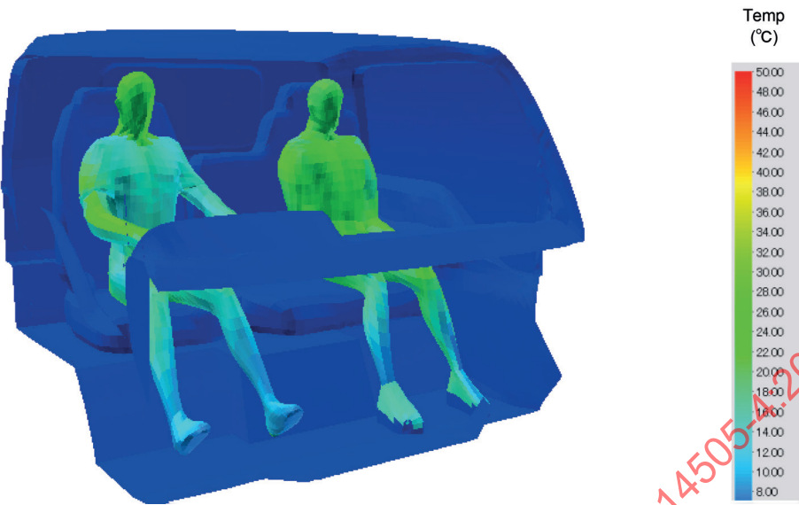
Figure B.6 — t_{eq} distribution close to body surfaces
