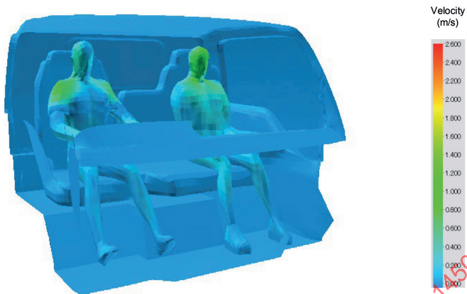
Figure B.4 — Velocity distribution close to body surfaces
